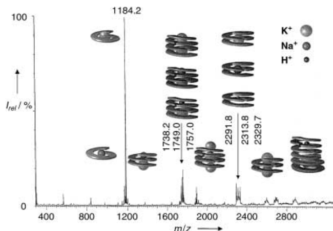
Figure 2. ES-MS spectrum of a 1/1 mixture of A n Bu and potassium picrate (2.7 mM in \text{CHCl}_3/\text{CH}_3\text{CN} (1.7/1.0)), 70 V. m/z : 1168.1 [ A +Na] ^+ , 1184.2 [ A +K] ^+ , 1176.4 [ 2A +K+Na] ^{2+} , 1738.2 [ 3A +K+H] ^{2+} , 1749.0 [ 3A +K+Na] ^{2+} , 1757.0 [ 3A +2K] ^{2+} , 1890.8 [ 3A +3K+Pic] ^{2+} , 2291.8 [ 2A +H] ^+ , 2313.8 [ 2A +Na] ^+ , 2329.7 [ 2A +K] ^+ , 2597.4 [ 2A +2K+Pic] ^+ , 2883.5 [ 5A +K+H] ^{2+} . The stacked structures shown are speculative, but agree with all the data obtained.
