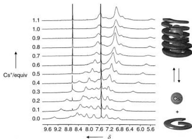
Figure 1. ^1\text{H} NMR titration of A n Bu (2.7 mM in \text{CDCl}_3/\text{CD}_3\text{CN} (1.7/1.0)) with cesium picrate (2.9 mM in the same mixture of solvents); right: representation of the formation of a stack of helical A n Bu components containing \text{Cs}^+ ions.
